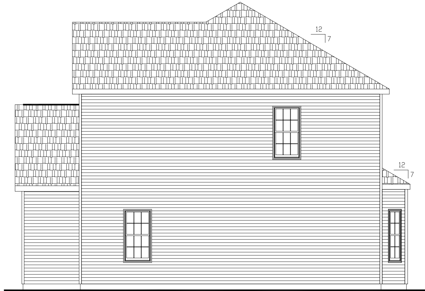
Gracin RIGHT ELEVATION ARCH STYLE GEORGIAN COLONIAL
